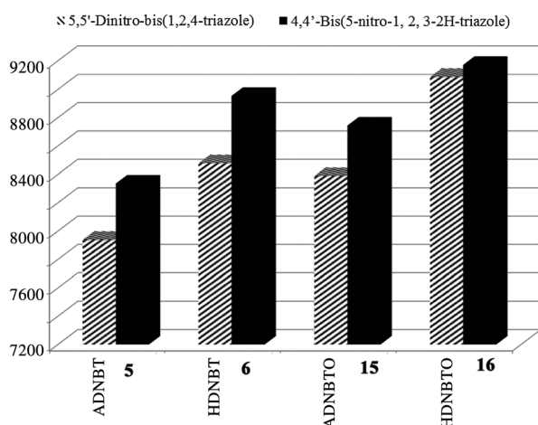
Figure 4. Bar diagram representation of the detonation velocities of isomers (A = ammonium salts, H = hydroxylammonium salts, DNBT = bistriazolate, DNBO = bistriazololate).
